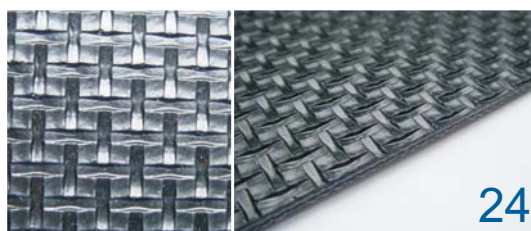
Name:Lattice Thickness:0.5mm Property:Incline conveying,medium friction Code:24 Width:3000mm
